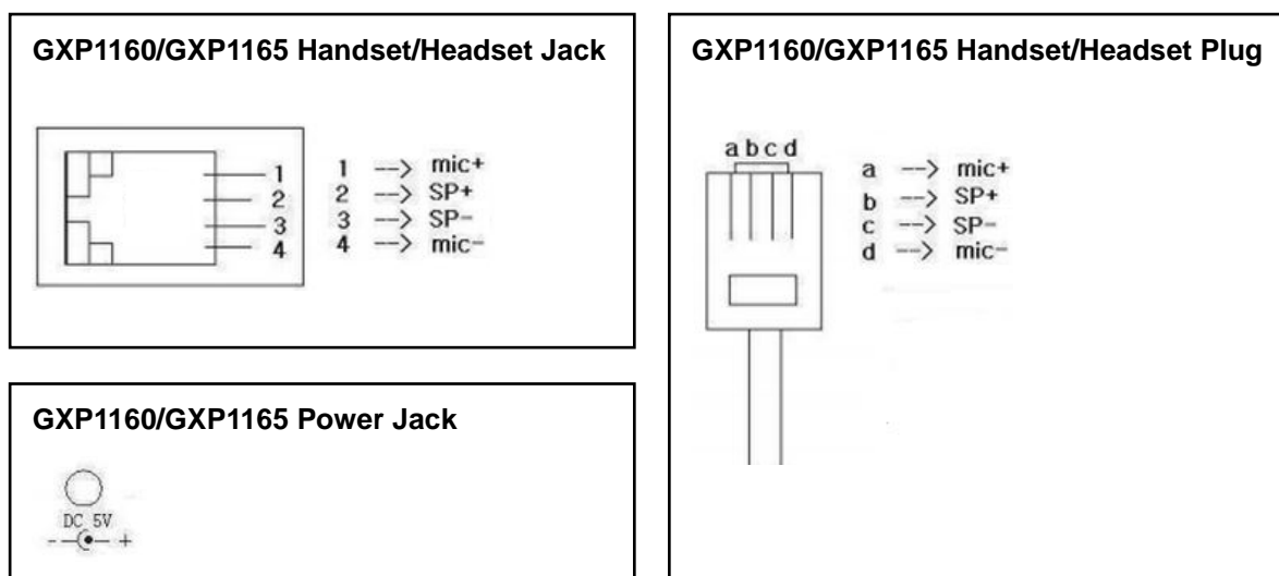
Figure 2: GXP1160/GXP1165 Pin-out
