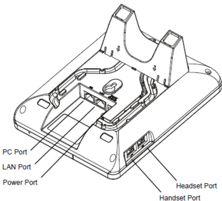
Figure 1: GXP1160/GXP1165 Ports
