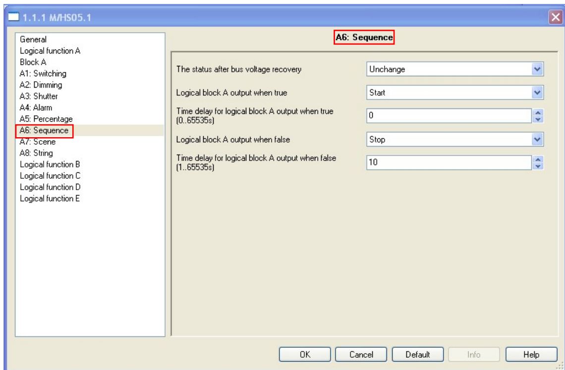
Fig3.6: “Sequence” parameter window ---The status after bus voltage recovery
