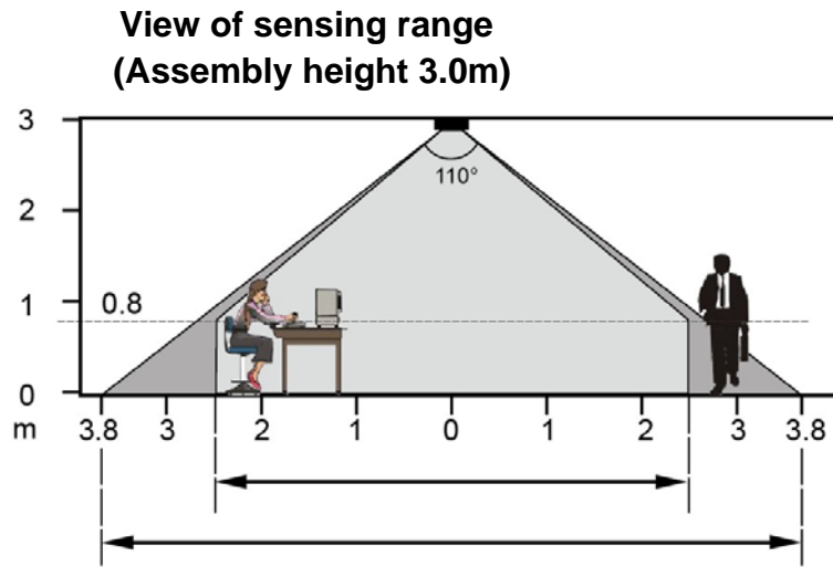
Side view of the sensing range
