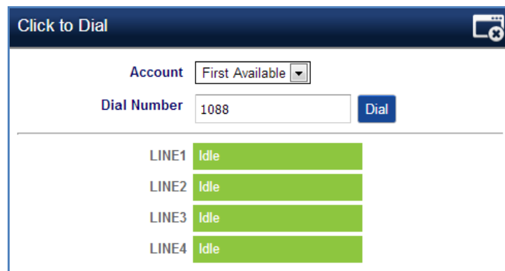
Figure 5: Click-to-Dial
